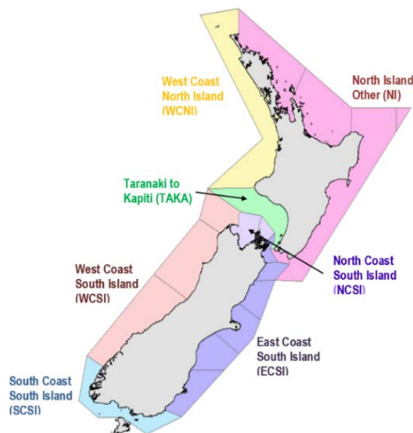
Figure 2: Spatial extent of sub-population areas delineating assessment sub-populations (discrete colours) and strata used to rescale habitat preference-based spatial abundance predictions of Hector's and Māui dolphins (black-edged polygons). Population sizes assumed for each sub-area are shown in Table 2. Note that the spatial abundance of Hector's and Māui dolphins was assumed to be zero at depths greater than 250 m, whereas the sub-population polygons depicted here extended an arbitrary distance from shore.
