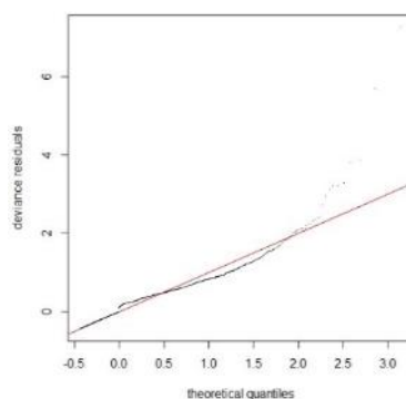
Figure 9: Quantile-quantile plot for models estimating the spatial abundance of Hector's dolphin, using the Ahuru model.
