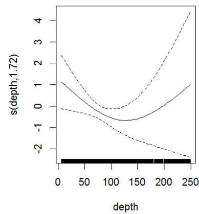
Figure A5-3 continued: Prey taxon GAM splines for all splined terms in a prey's respective final model.
