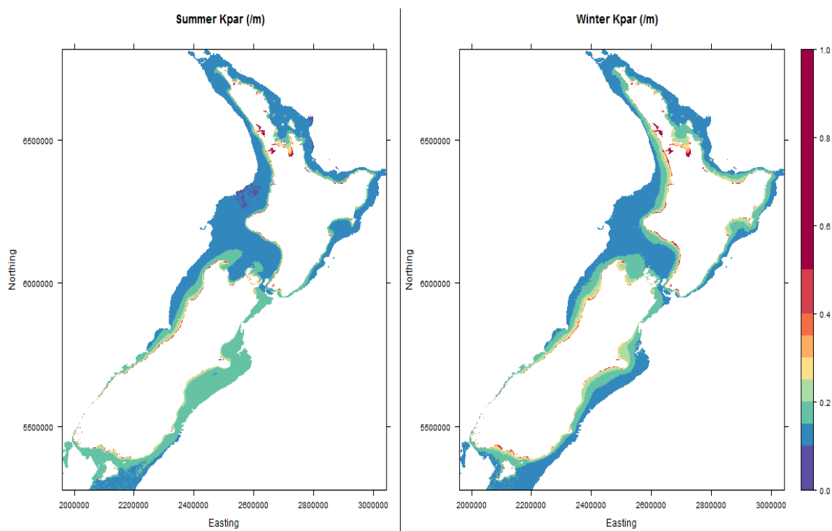
Figure A6-5: Seasonal downwelling light attenuation ( K_{\text{PAR}} \text{ m}^{-1} ), used in Hector's/Māui distribution modelling.
