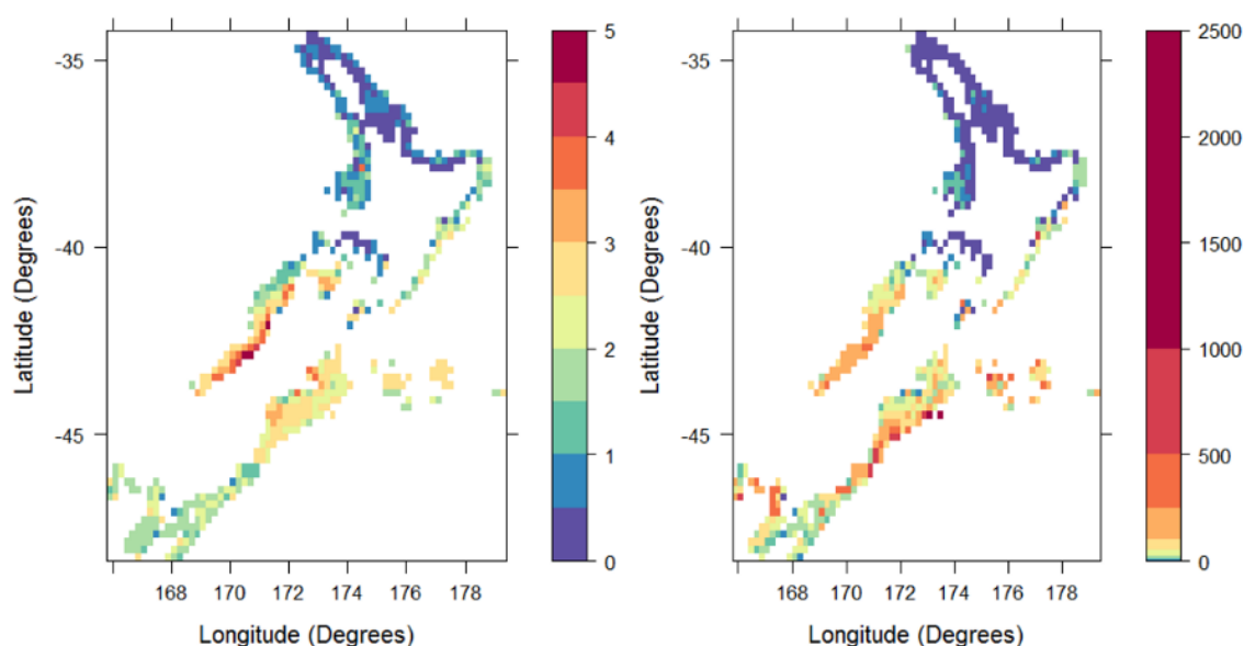
Figure 26: Unstandardised mean count of species (left) and combined biomass in kg (right) of the six key prey taxa by diet mass (Miller et al. 2013 and Table A5-2) for combined Kaharoa and Tangaroa survey stations aggregated by 0.2-degree grid.
