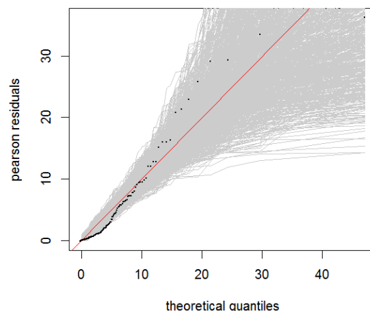
Figure 14: Simulation-based quantile-quantile plots GAMs fitting to public sightings with Pearson residuals and 200 simulation replicates.
