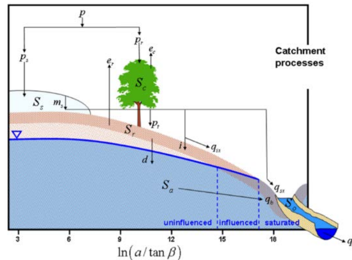
Figure A9-3: TopNet model structure within each sub-basin, showing modelled water fluxes and storages.
