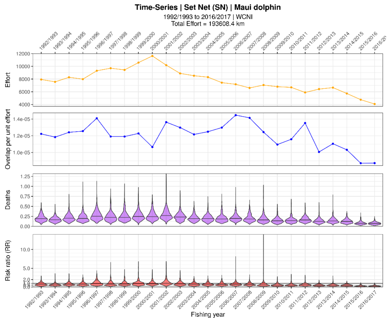
Figure A16-2: Commercial set net effort by fishing year (top) and spatial risk model outputs for Māui dolphins also by fishing year: spatial overlap, annual deaths and risk ratio. This model run assumed a calibration coefficient ( \phi ) of 0.2.
