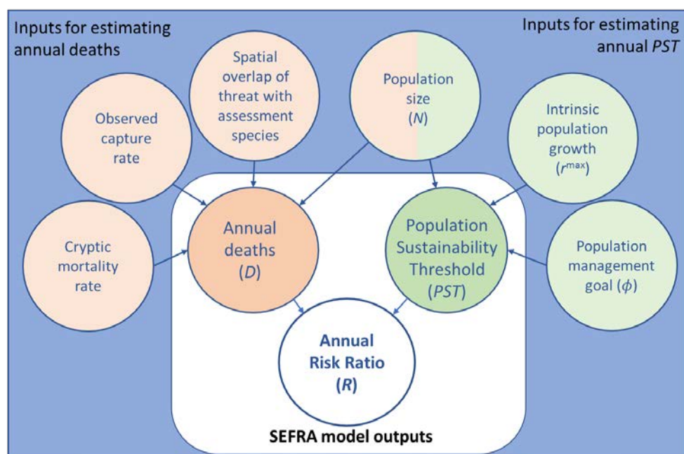
Figure 1: Conceptual diagram of spatially-explicit risk model approach and data inputs. Note that the population size is used in both the derivation of annual deaths and the Population Sustainability Threshold (PST).
