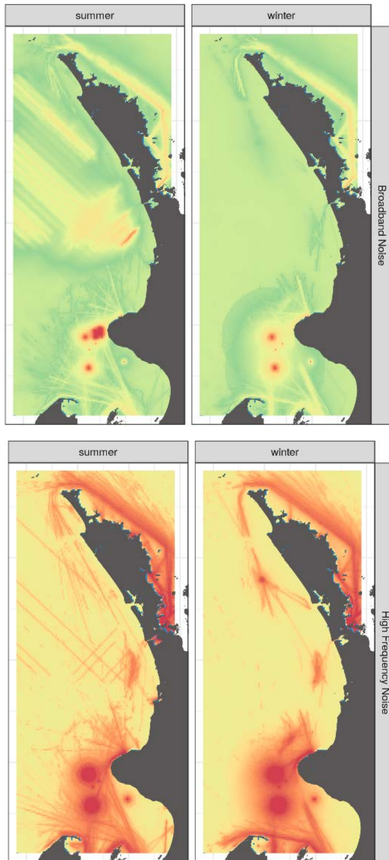
Figure A11-6: Estimated cumulative broadband noise (top) and high-frequency noise (bottom) in summer (left) and winter (right). Spatial estimates from noise modelling by McPherson et al. (2019).
