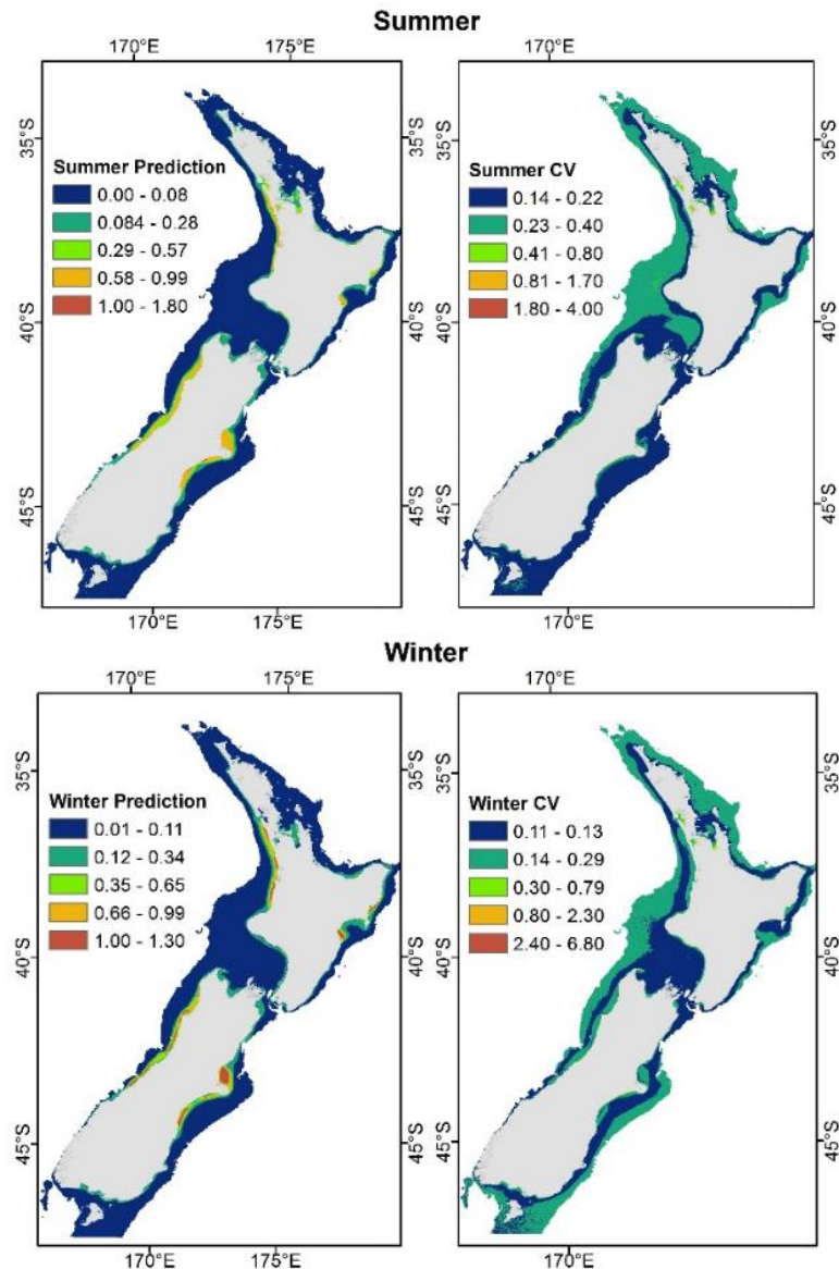
Figure 11: Predicted spatial abundance (left) and spatial CV associated with the prediction (right) of Hector's/Māui dolphins in summer (top) and winter (bottom) from the Ahuru model.
