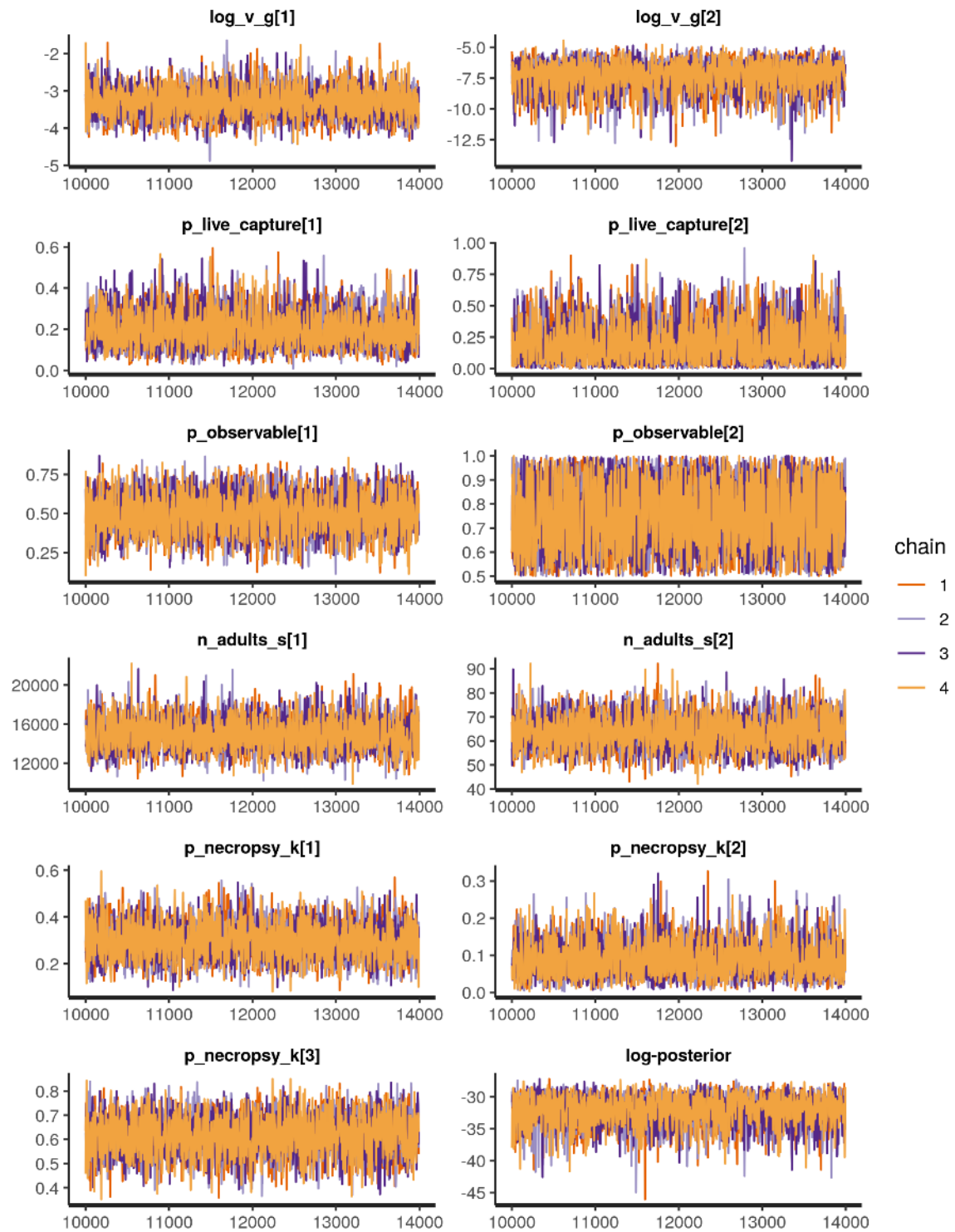
Figure A13-1: Markov chain Monte Carlo (MCMC) trace plots for all estimated model parameters and the log-posterior density (i.e. the objective function). This model run assumed a calibration coefficient ( \phi ) of 0.2.
