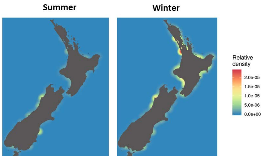
Figure A9-6: Estimated relative coastal water densities of Toxoplasma gondii oocysts in summer (left) and winter (right).
