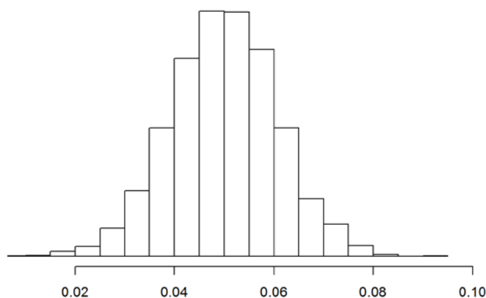
Figure A2-1: Posterior distribution of r^{\max} using the model developed by Edwards et al. (2018), updated with supplementary ageing and maturity stage information shown in Appendix 1.
