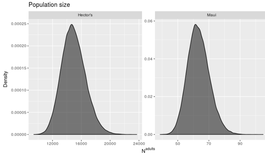
Figure 3: Population size ( N_s ) priors for Hector's and Māui dolphins.
