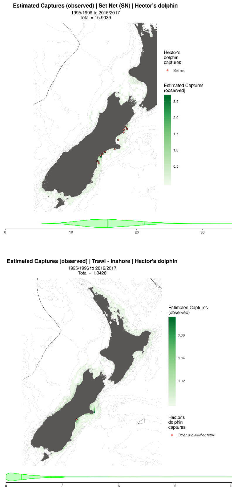
Figure A15-3: Predicted number of observed Hector's dolphin captures from 1995/96 to 2016/17. Observed Hector's dolphin captures in set nets between 1995/96 to 2016/17 are also shown as red points. The posterior distribution of the total estimated observed number of captures is also displayed as the violin along the bottom with the median and upper 90% quantile indicated by the vertical lines within the violin.
