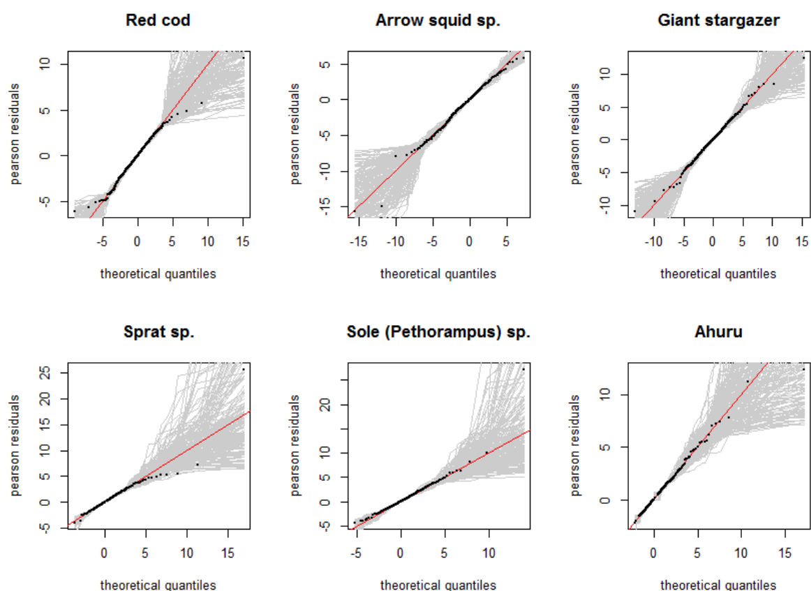
Figure A5-2: Simulation-based quantile-quantile plots for final prey species GAMs, with Pearson residuals and 200 simulation replicates.
