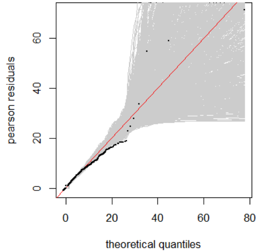
Figure A8-2: Simulation-based quantile-quantile plot for final broadnose sevengill shark GAM, with Pearson residuals and 1000 simulation replicates.
