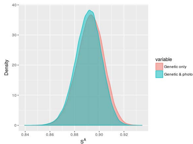
Figure 6: Non-calf annual survival ( S_s^{1+} ) prior for Māui dolphins. The estimate using genetic mark-recapture observations only “Genetic only” (i.e. not photo-based mark-ID also) was used for all model runs.
