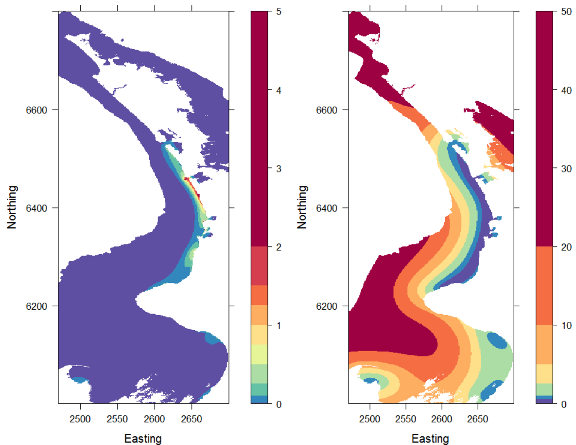
Figure 16: Estimated spatial density (left) and spatial CV associated with this model prediction (right) of Hector's/Māui dolphins off the coast of the North Island using model fitting to public sightings
