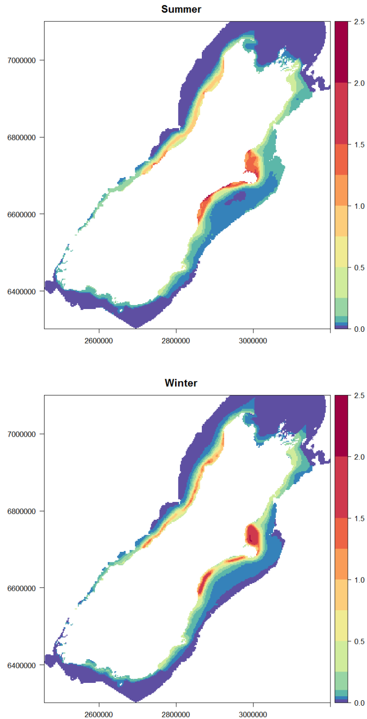
Figure 17: Final seasonal estimated spatial density of Hector's and Māui dolphins used for spatial risk assessment—South Island.
