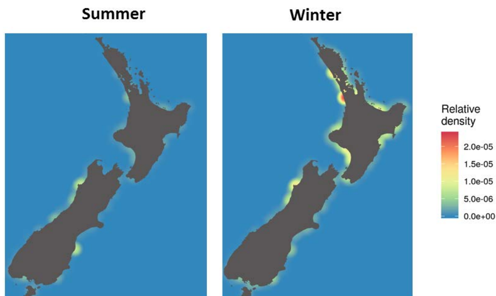
Figure 28: Estimated relative coastal water densities of Toxoplasma gondii oocysts in summer (left) and winter (right).
