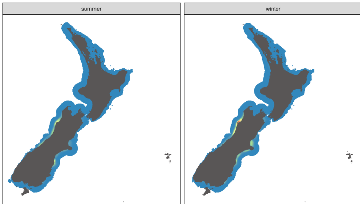
Figure A12-1: Toxoplasmosis estimated seasonal spatial overlap with Hector's and Māui dolphins.
