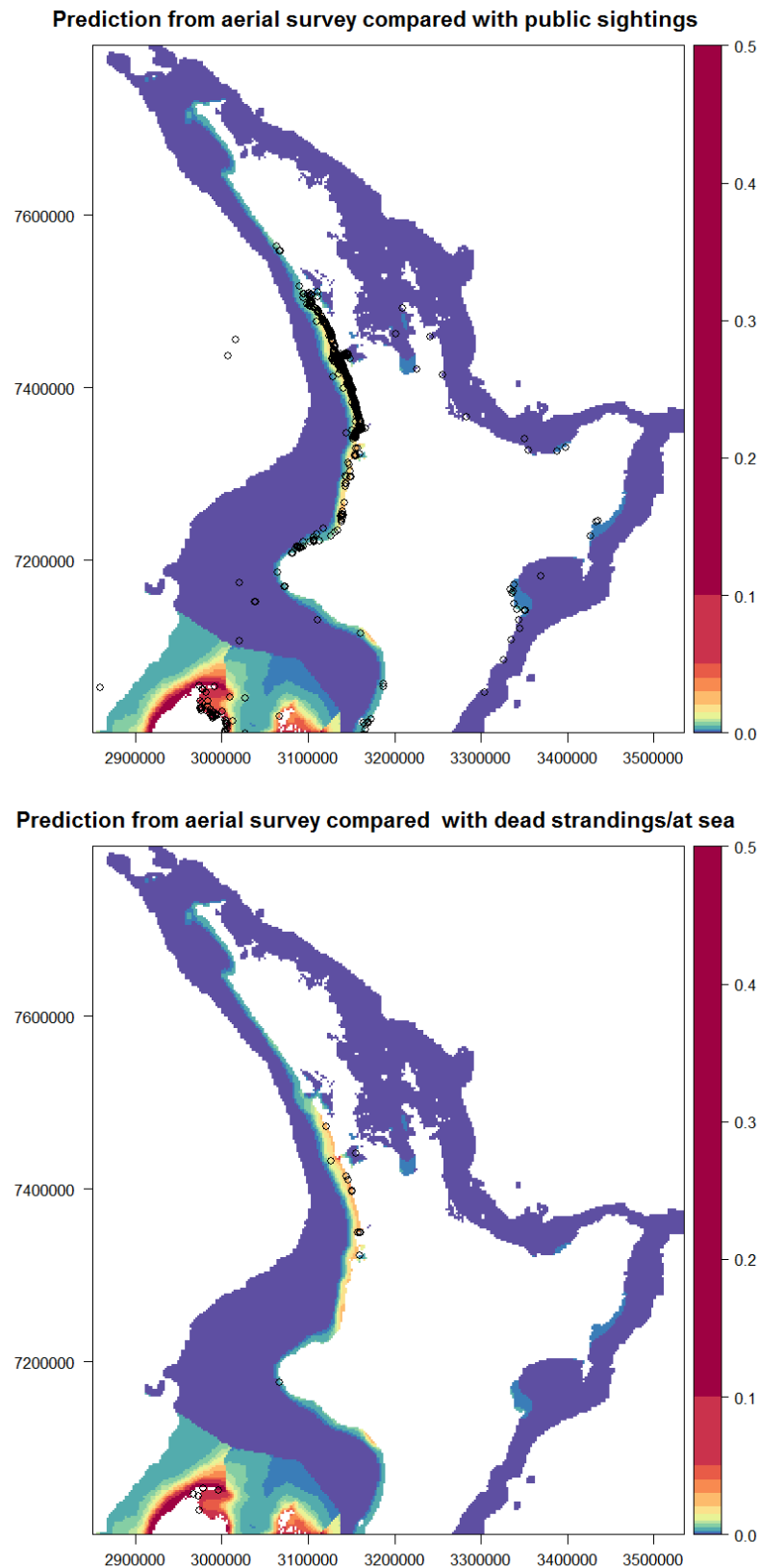
Figure A7-3: Final predicted spatial abundance of Hector's and Māui dolphins in summer used for the spatial risk assessment compared with the spatial distribution of public sightings of live animals, including unvalidated sightings (top) and sightings of dead animals (stranded and at-sea)—North Island.
