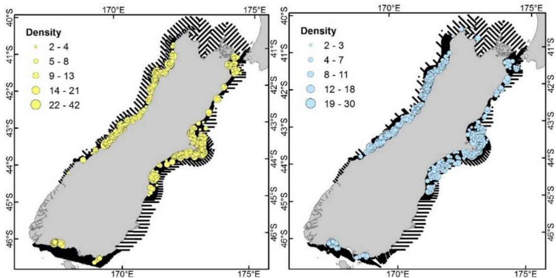
Figure 7: Aerial survey effort (black lines) and Hector's dolphin density estimates for summer (yellow, left panel) and winter (blue, right panel) aerial surveys. Size of circles represents estimated number of Hector's dolphins per 1-km survey transect segment.
