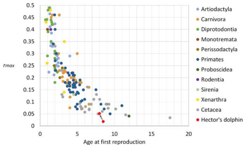
Figure 24: Comparative plot of r^{\max} against age at first reproduction (AFR) for a variety of mammalian orders (Duncan et al. 2007). For Hector's dolphin, both the previous and updated values are shown (red points with an arrow between). The updated value of r^{\max} derived here for Hector's dolphin is now consistent with that expected from other mammals, given estimated age at first reproduction.
