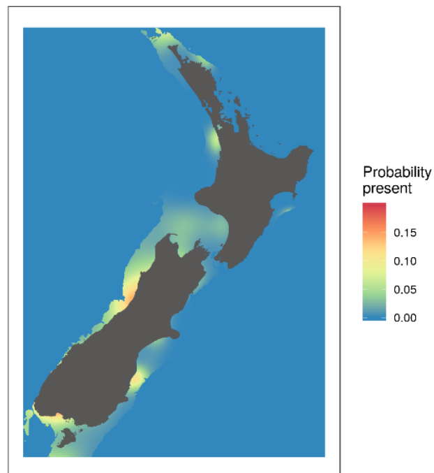
Figure A11-2: Predation (broadnose sevengill shark) estimated spatial threat intensity.
