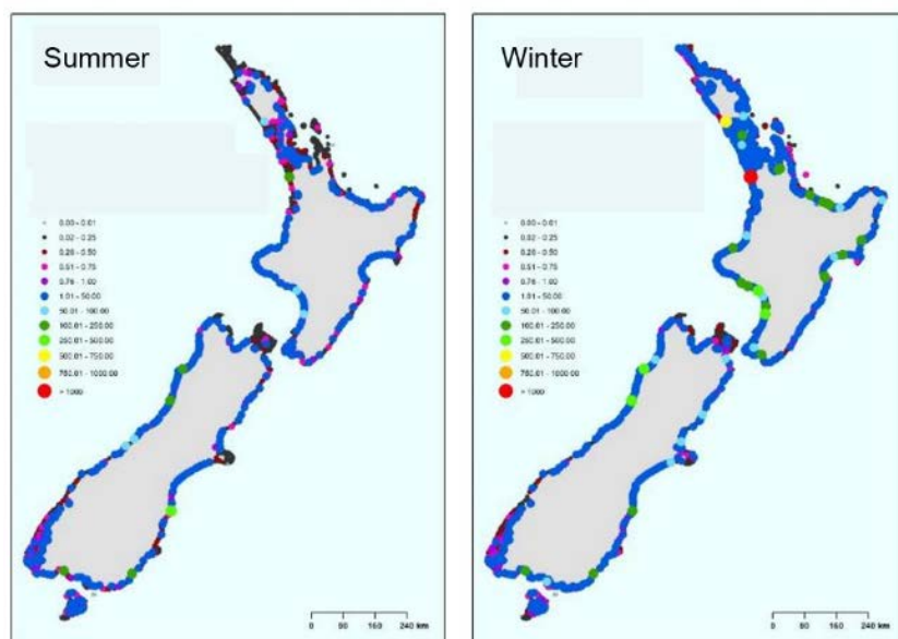
Figure A9-5: Estimated load of Toxoplasma gondii oocysts at terminal outflow points of New Zealand rivers in summer (left) and winter (right), relative to the annual mean across all terminal river outflows.
