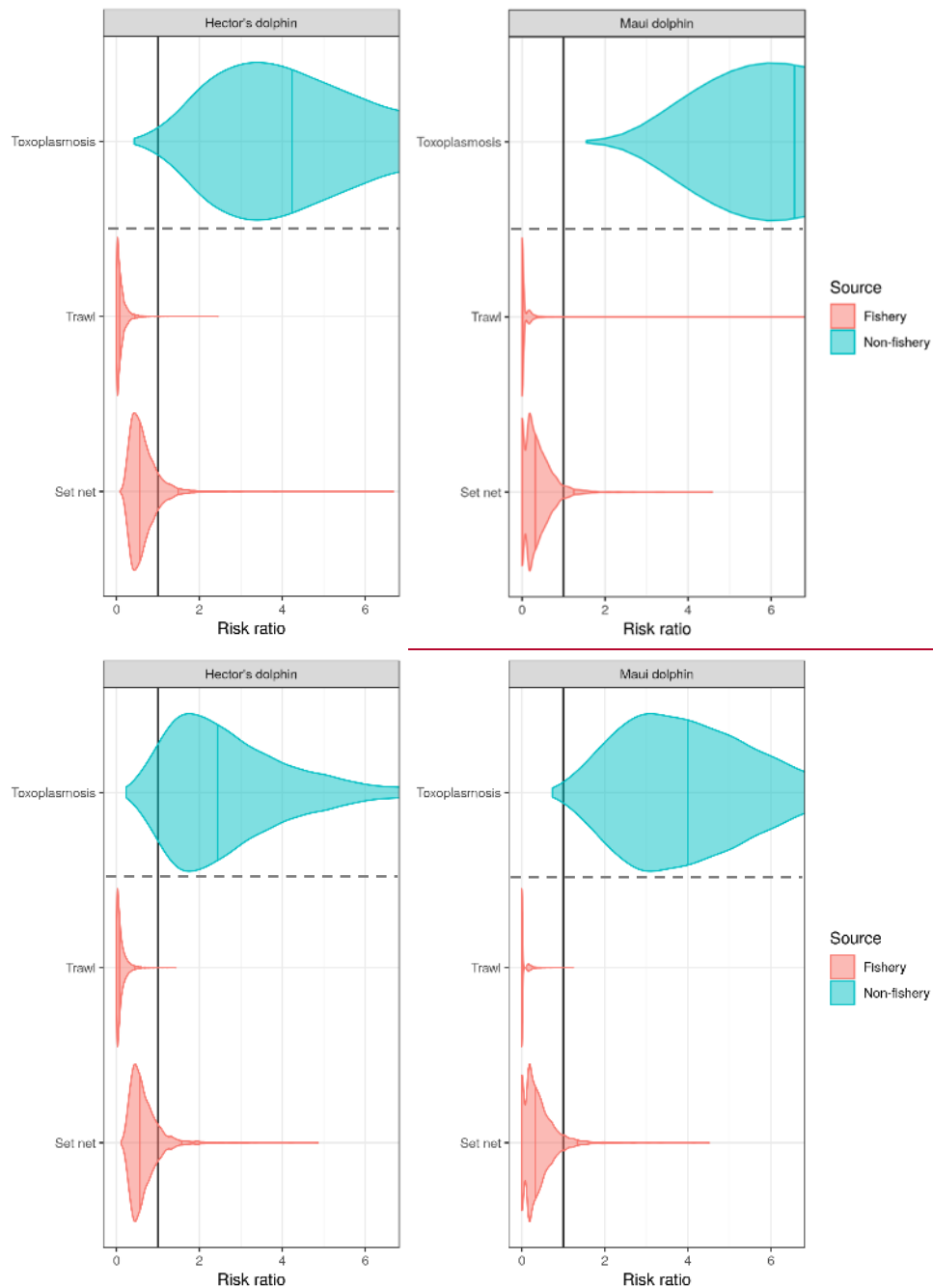
Figure 22: Annual commercial fishery (set net and inshore trawl) and toxoplasmosis risk ratios for Hector's dolphins (left) and Māui dolphins (right), assuming equal detection probability of non-fishery causes of death (top), or a ten-fold reduction in the relative detection probability of predation mortality (bottom). The median and 97.5% quantile are indicated as vertical lines within each density. Dashed lines delineate threats for which differing methods were used to estimate annual risk ratio (above the line = based on proportions in the necropsied sample; below the line = using observer and vessel-reported commercial fishery data).
