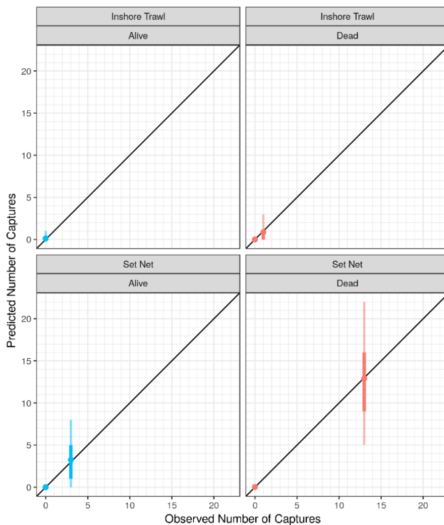
Figure A13-3: Observed vs. spatial risk model predicted number of Hector's/Māui dolphin captures that are alive (blue) or dead (red) in inshore trawl or set nets. This model run assumed a calibration coefficient ( \phi ) of 0.2.
