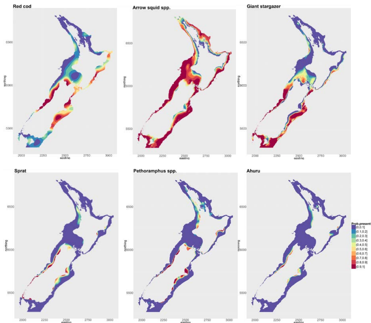
Figure A5-5: Model predicted proportion of Kaharoa and Tangaroa survey stations in which key prey species (Table A5-2) were present.
