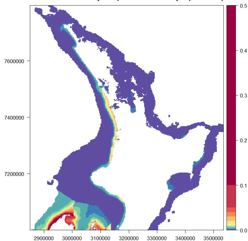
Figure A7-4: Final predicted spatial abundance of Hector's and Māui dolphins in summer used for the spatial risk assessment compared with the spatial distribution of commercial fishery observer sightings (top) and commercial fishery-reported captures (set net and trawl)—North Island.
