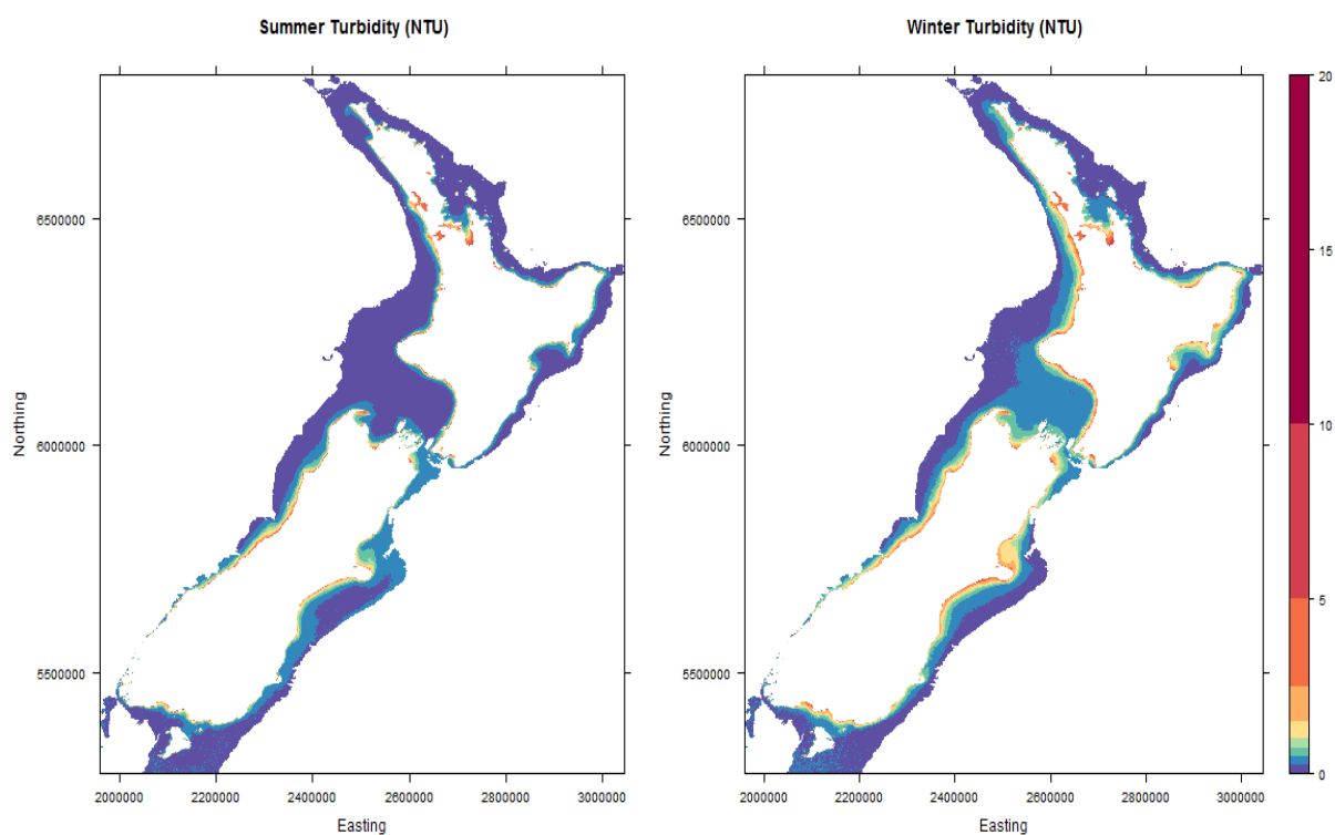
Figure A6-2: Seasonal turbidity – Nephelometric Turbidity Units (NTU), used in Hector’s/Māui distribution modelling.
