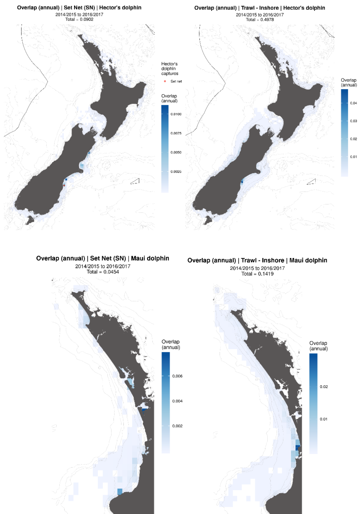
Figure A15-5: Total annual overlap (observed and unobserved) from 2014/15 to 2016/17. Observed Hector's dolphin captures in set nets between 2014/15 to 2016/17 are also shown as red points.
