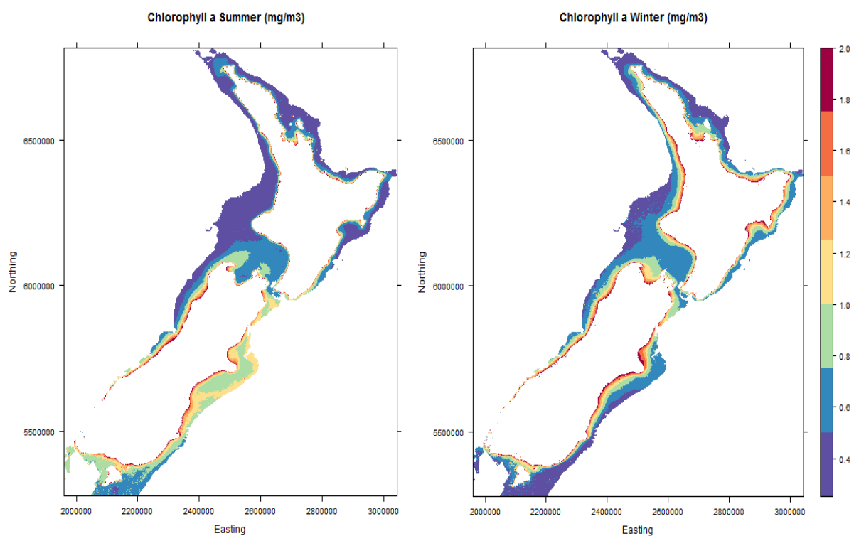
Figure A6-4: Seasonal Chlorophyll a ( \text{mg}/\text{m}^3 ), used in Hector's/Māui distribution modelling.
