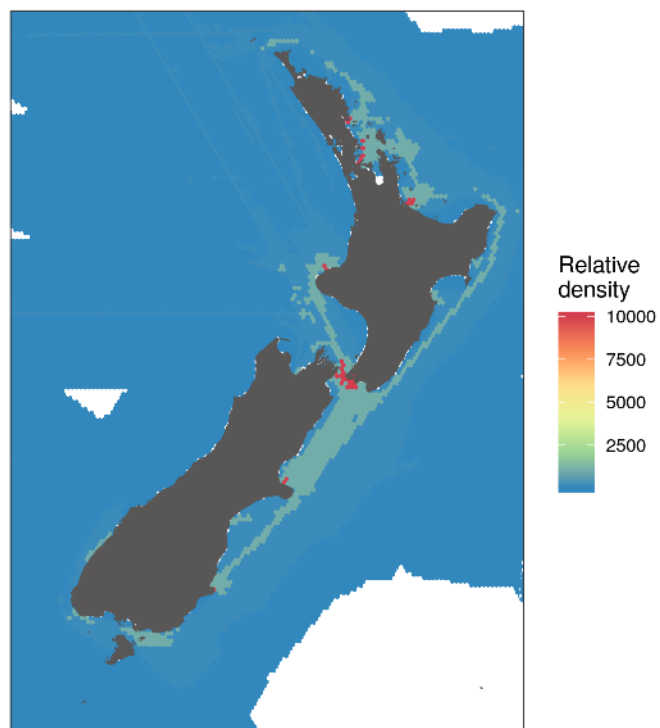
Figure A11-5: Oil spill risk estimated spatial threat intensity.
