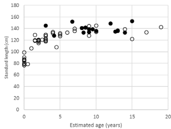
Figure A1-2: Standard length-at-age of all female Hector's/Māui dolphins; used for estimation of r^{\max} by Edwards et al. (2018). Black circles are estimates from supplementary sampling, open circles are measurements and previous estimates (Duignan et al. 2003, Duignan et al. 2004, Duignan & Jones 2005, Slooten 1991).
