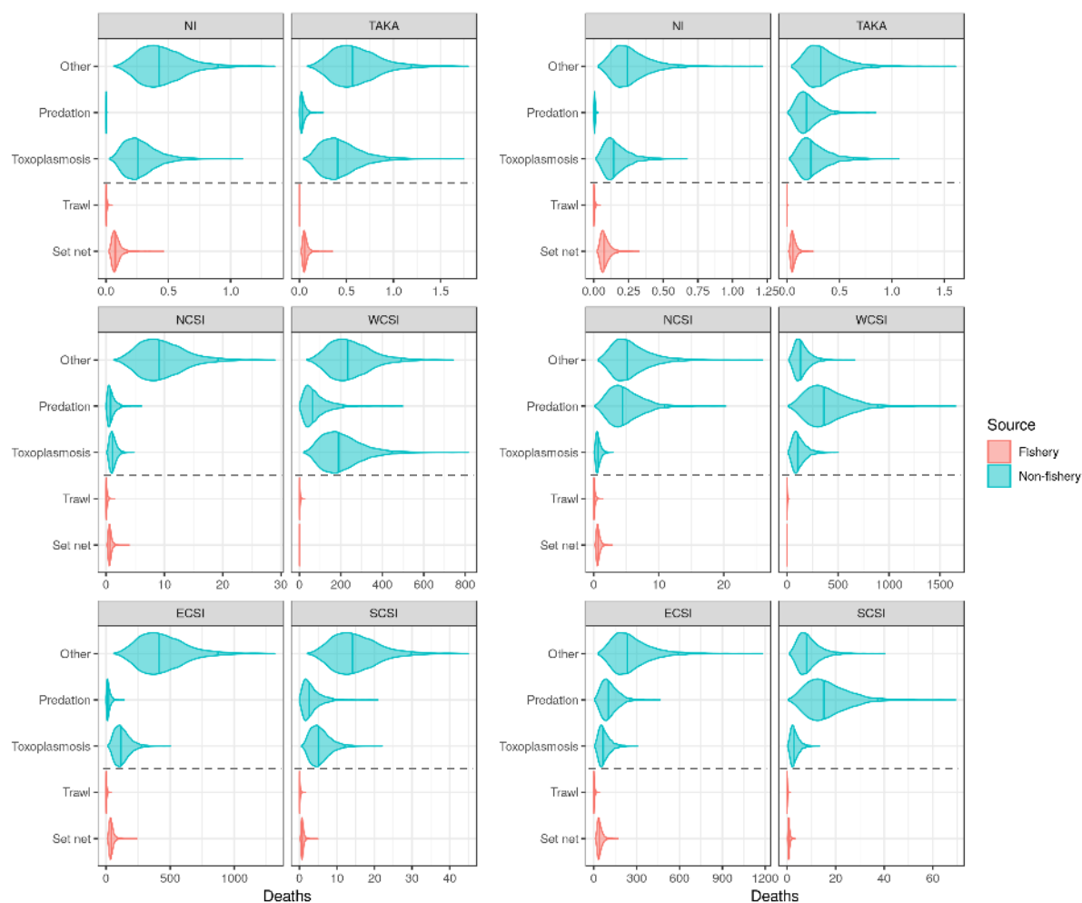
Figure 21: Annual estimated commercial fishery (set net and inshore trawl) and non-fishery (toxoplasmosis, predation and other) deaths for Hector's dolphins by sub-population or summary area (defined in Table 2), assuming equal detection probability of non-fishery causes of death (left-hand panel of plots), or a ten-fold reduction in the relative detection probability of predation mortality right-hand panel of plots). The median and 97.5% quantile are indicated as vertical lines within each density. Dashed lines delineate threats for which differing methods were used to estimate annual deaths (above the line = based on proportions in the necropsied sample; below the line = using observer and vessel-reported commercial fishery data).
