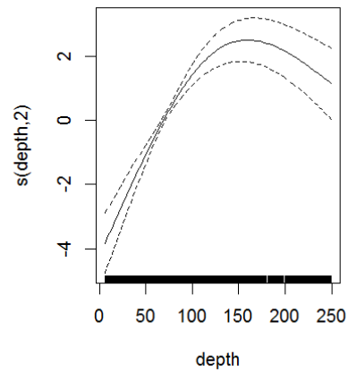
Figure A5-3: Prey taxon GAM splines for all splined terms in a prey's respective final model.
