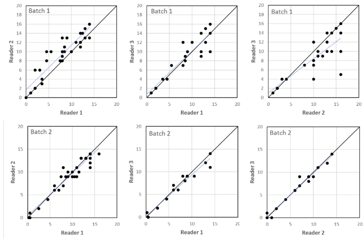
Figure A1-1: Pairwise comparison of reader estimates comparing all three readers separately for sample Batch 1 (top) and Batch 2 (bottom). Note consistent positive bias with estimates for Reader 2 in Batch 1, which was not apparent in Batch 2. The solid line highlights the relationship that would occur with perfect agreement between reader estimates. The dotted blue line highlights the linear trendline between reader estimates.
