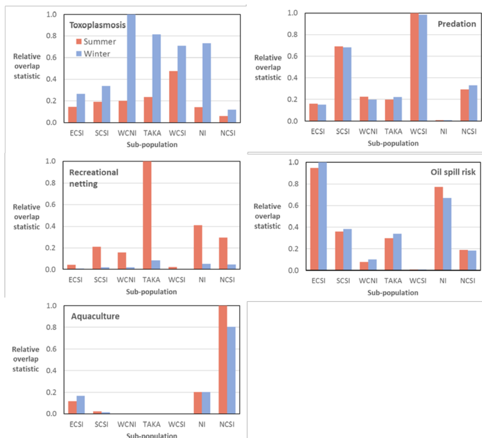
Figure 19: Relative overlap statistic between threats and Hector's/Māui dolphins by threat, subpopulation and season. Rescaled as a proportion of the maximum value for a respective threat across all sub-populations and season. A graphical representation of the same estimates in Table 14.
