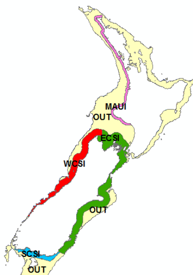
Figure 12: Spatial extent of areas used by the Hector’s dolphin habitat model to estimate potential habitat capacity given the available habitat in each area (see Table 8). Area label notation was as follows: “WCSI” = West Coast South Island; “ECSI” = East Coast South Island; “SCSI” = South Coast South Island; “MĀUI” = West Coast North Island (could comprise Hector’s or Māui dolphins across this area); “OUT” = all other grid cells out to a depth of 250 m. Note that these areas do not correspond with those used to define sub-populations used by the SEFRA model (Figure 2).
