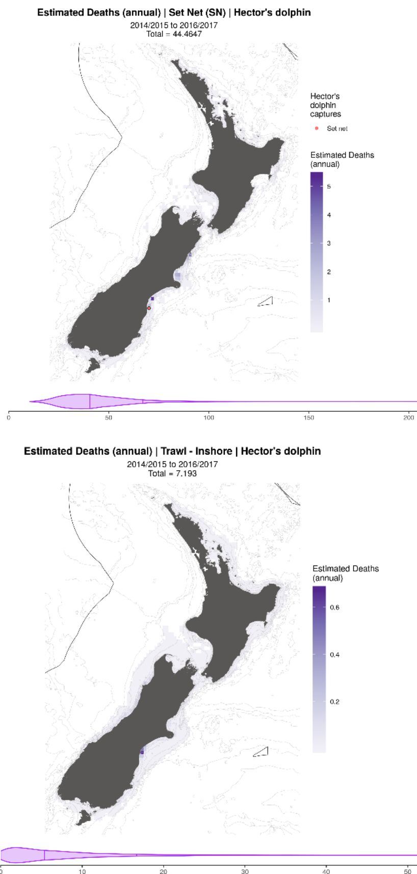
Figure A15-6: Total annual deaths (the mean from 2014/15 to 2016/17). Observed Hector's dolphin captures in set nets between 2014/15 and 2016/17 are also shown as red points. The posterior distribution of the number of deaths is also displayed as the violin along the bottom with the median and upper 90% quantile indicated by the vertical lines within the violin.
