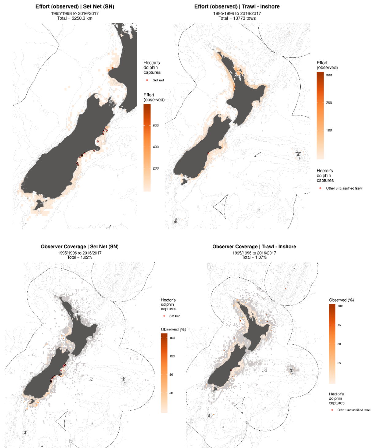
Figure A15-1: Total observed set net (top left) and inshore trawl (top right) fishing effort and observer coverage (bottom) in New Zealand from 1995/96 to 2016/17. Grey pixels represent cells where there was effort but no observer coverage. Observed Hector's dolphin captures in set nets and trawls between 1995/96 to 2016/17 are also shown as red points.
