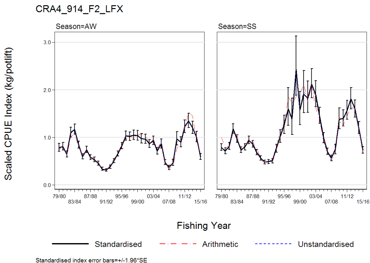
Figure A.15. Scaled standardised F2_LFX CPUE (kg/potlift) by period for the Area 914 CRA 4 sub-stock with the AW-SS seasons plotted separately. Also shown are the arithmetic or “raw” CPUE series and the geometric mean of the CPUE (“unstandardised”). The standardised and unstandardised series were scaled by multiplying each index in the unscaled series (where the geometric mean=1) by the geometric mean of the arithmetic CPUE series for each seasonal category (geometric mean for AW=0.74 kg/potlift; geometric mean for SS=1.04 kg/potlift).
