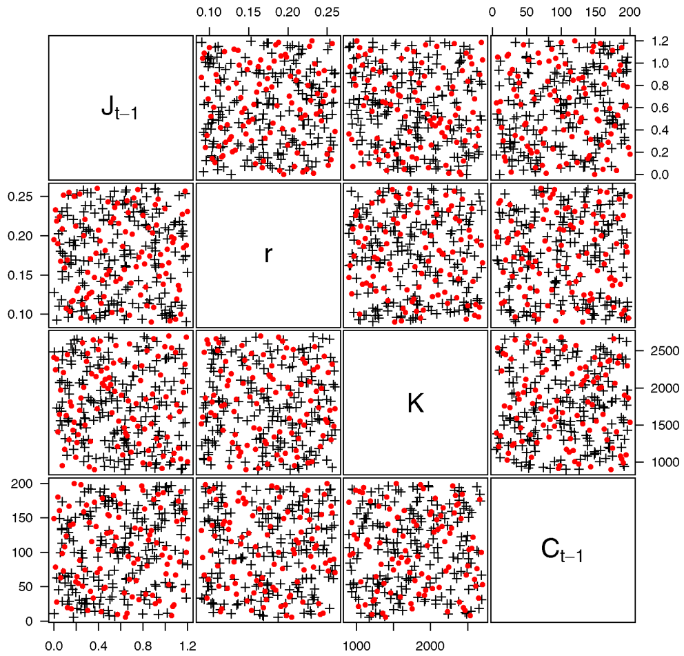
Figure 7.5: Points (•) were used to condition the emulator, crosses (+) used to test the performance of the emulator.
